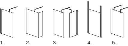
1. Single screen / 2. Single screen with return / 3. Two screens combined / 4. Single screen with one or two posts / 5. Single screen with two arms.
