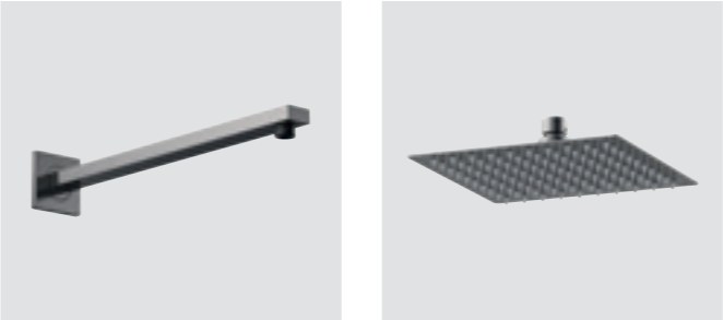
Square Wall Mounted Shower Arm L360 x W30mm ARM713 £143.00 Square Fixed Head 200 x 200mm A7088 £130.00 MP
