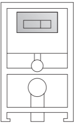
Dual Flush Concealed WC Cistern with Mid-Height Wall Hung Frame H820 - 880 x W515 max x D150 - 200mm XTY007 £527.00
