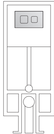
Dual Flush Concealed WC Cistern with Wall Hung Frame H1136-1336 x W520mm With Square Buttons XTY009S £310.00 With Round Buttons XTY009R £310.00
